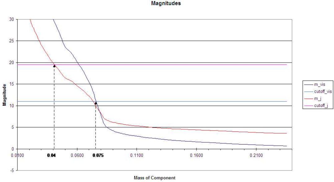
Figure 1. Magnitude versus Mass graph for Nemesis for a assumed period of 27 MYr. The horizontal lines indicate the IR and optical catalogue limits
