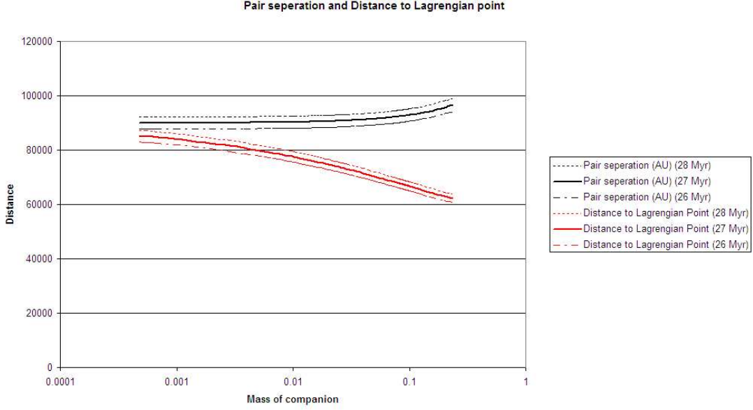
Figure 2. Distance from the Sun to L1 and to Nemesis as a function of mass of Nemesis, for values of the orbital period of nemesis as 26 Myr, 27 Myr and 28 Myr.
