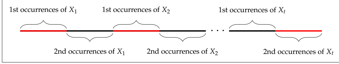
Figure 3: A 2-regularly-interleaving sequence.
